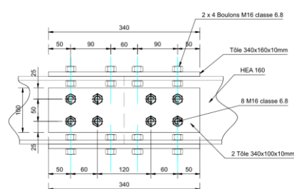
Detail Eclisse HEA 160
